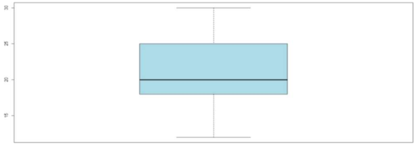
Outlier Detection
